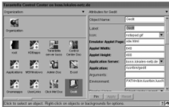
Abbildung 11.26: Tarantella Control Center – Organization
